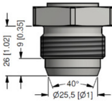
G1" Konus, SW41
