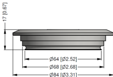
Varivent® DN 40/50
