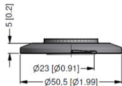
Clamp DN 25 / 1" (DIN 32676) p N ≤ 16 bar
