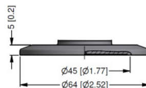
Clamp DN 50 / 2" (DIN 32676) p N ≤ 16 bar
